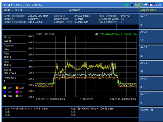
RFoCPRI — Spectrum
